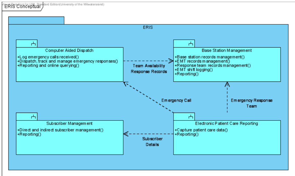
Figure 2: ERIS Package Diagram
