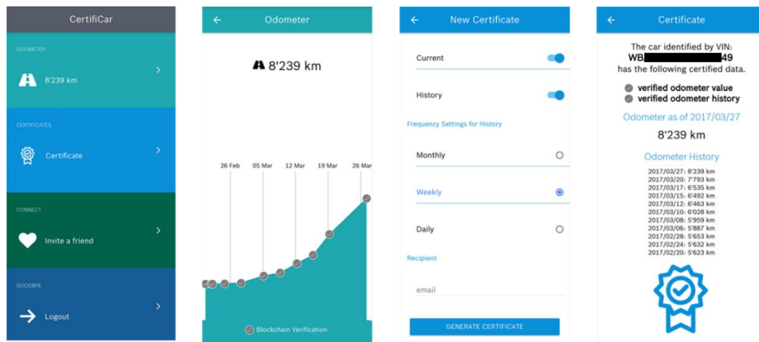
Figure 10. The Main Screens of the Smartphone Application
