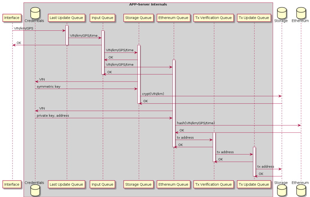
Figure A-2. Queue Management in the Final Version of the Application
