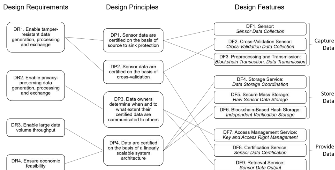
Figure 3. Design Requirements, Principles, and Features
