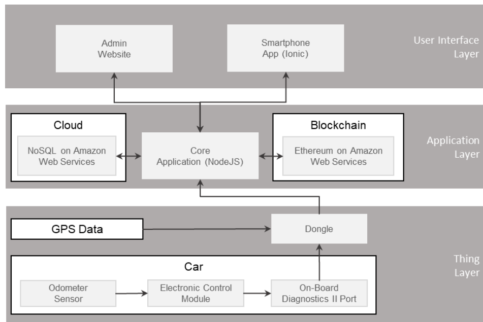
Figure 6. Prototype Architecture
