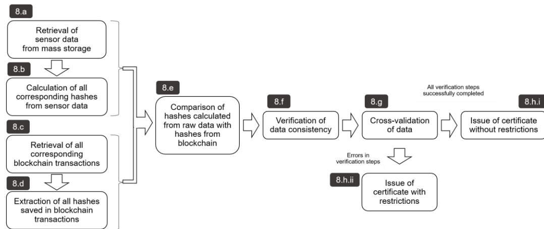
Figure 5. A Detailed View of the Certification Process
