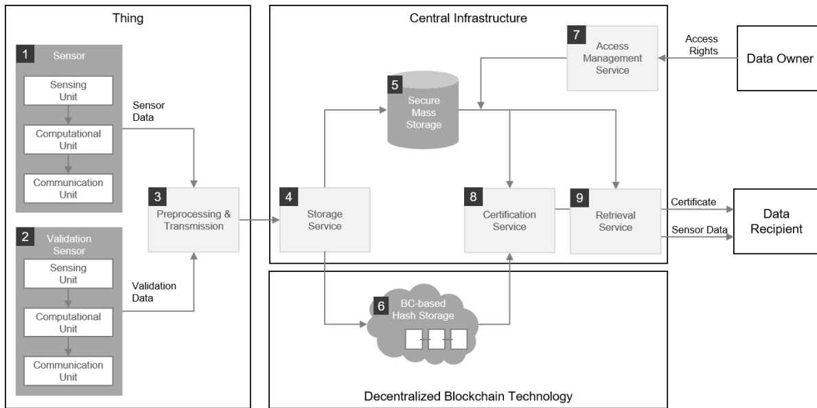
Figure 4. Artifact Architecture
