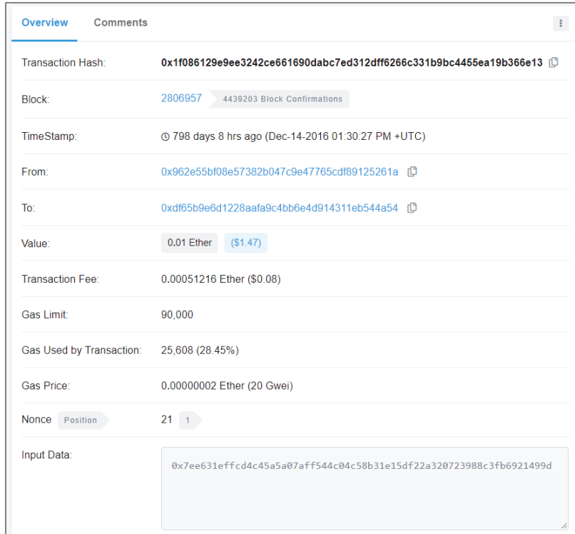
Figure 8. Transaction of Figure 7 on etherscan.io with the Ether Price at the Time of the Transaction
