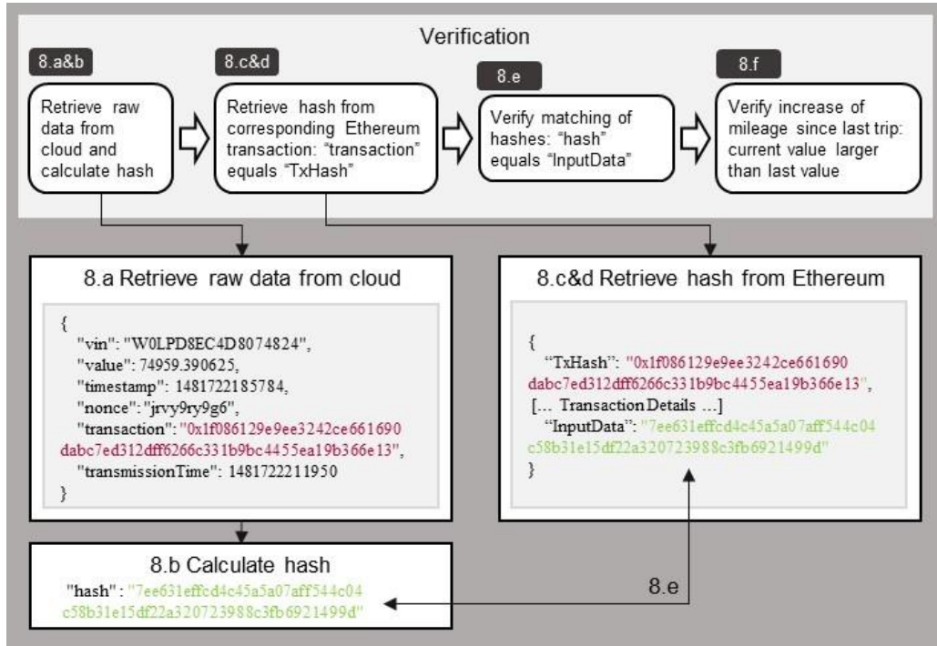
Figure 9. First Implementation of the Verification Process (Hashes in ASCII Format to Increase Readability)
