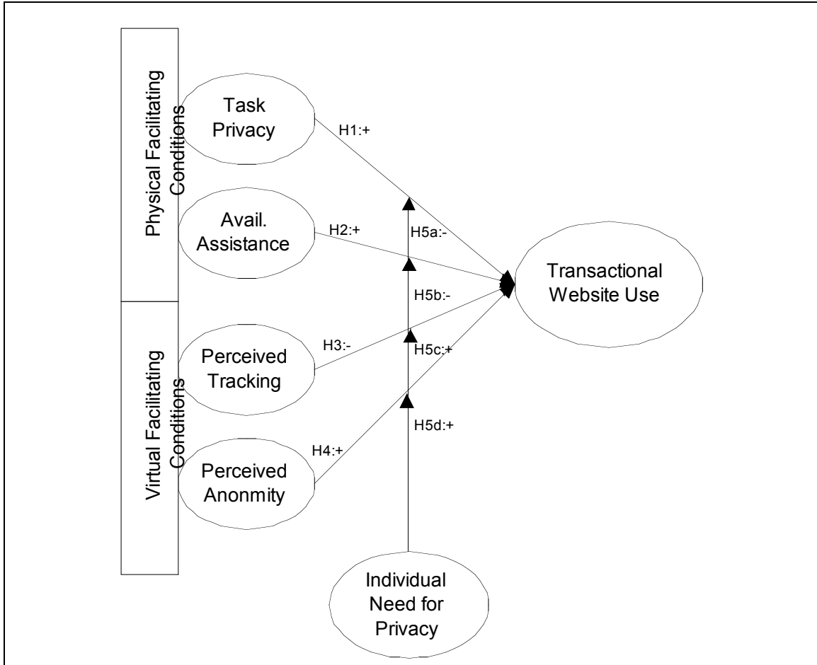
Figure 2: Research Model
