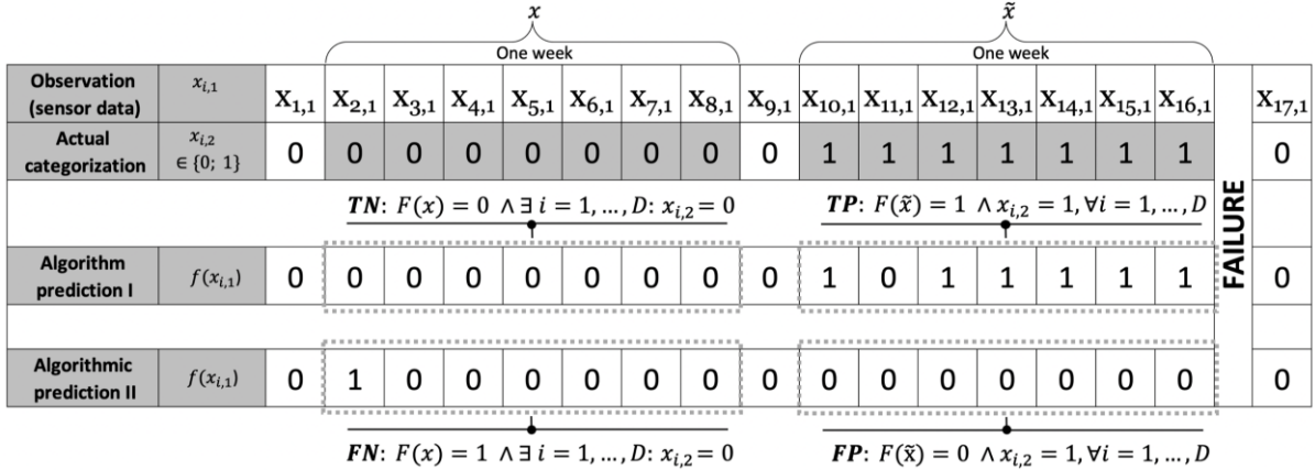
Figure 2. Four PdM model states in an example of 17 observations
