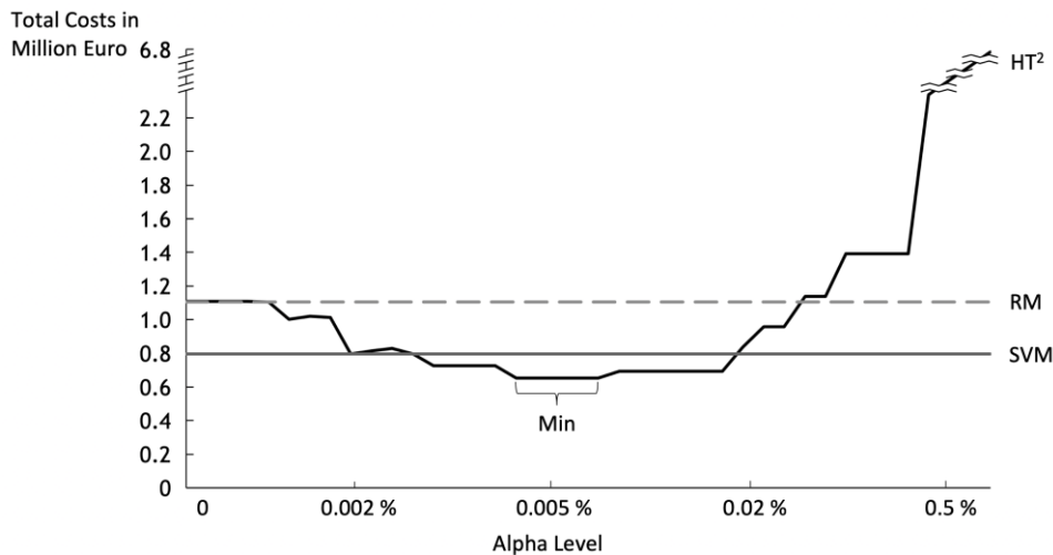
Figure 3. Total costs depending on the alpha level for SVM, HT 2 , and RM
