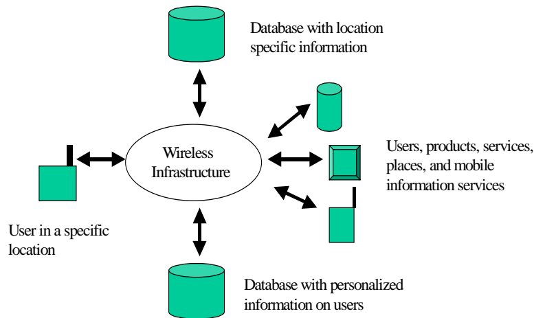
Figure 1. Location-based Services
