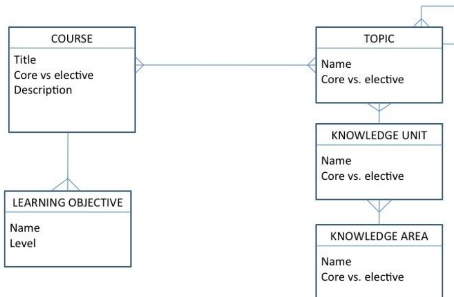
Figure 5: Simplified Curriculum Architecture Model
