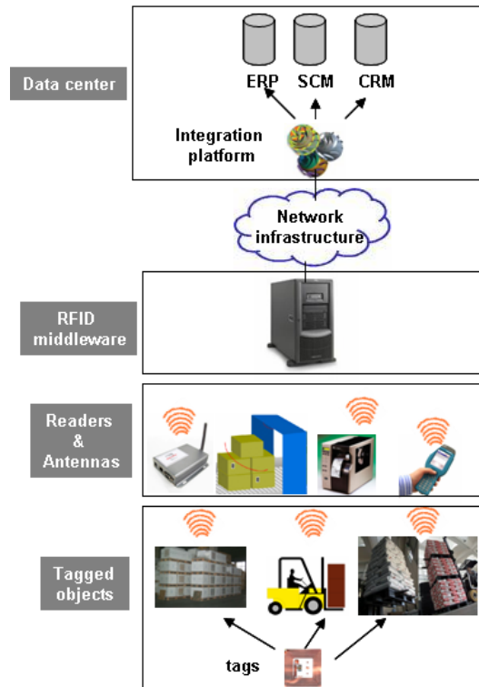
Figure 4. Typical RFID System Components
