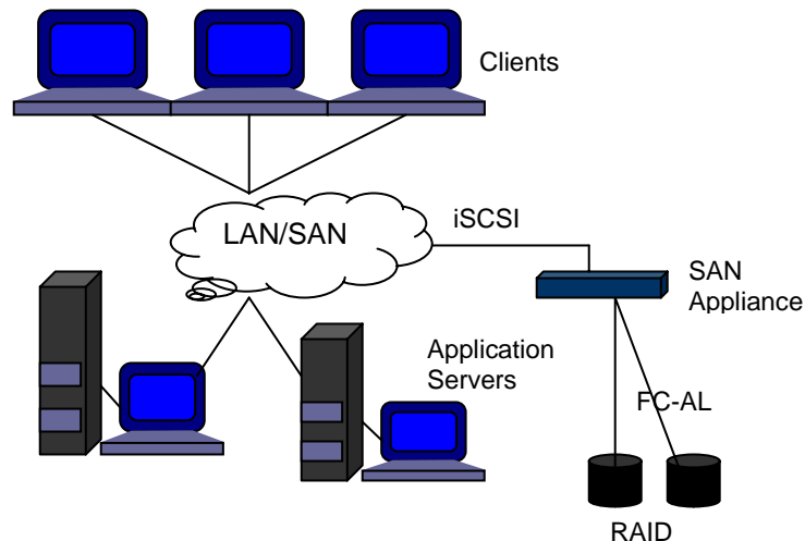
Figure 6. IP-based SAN
