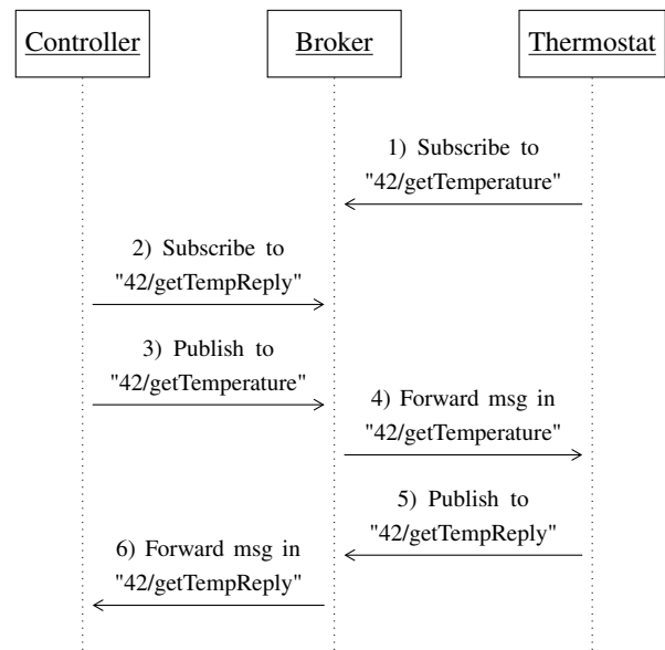
Fig. 2. Interaction in the home automation example in MQTT.
