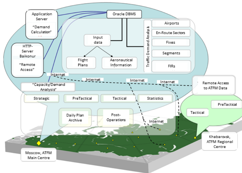
Figure 2. Russian Air Traffic Flow Management System Architecture
