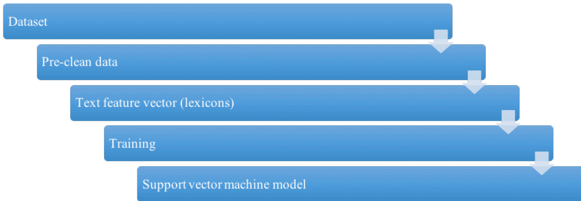
Figure 2. Analysis Procedure
