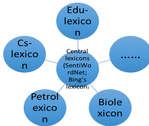
Figure 1. Lexicon Network
