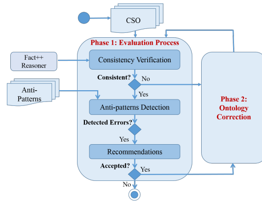
Figure 4. Ontology evaluation approach
