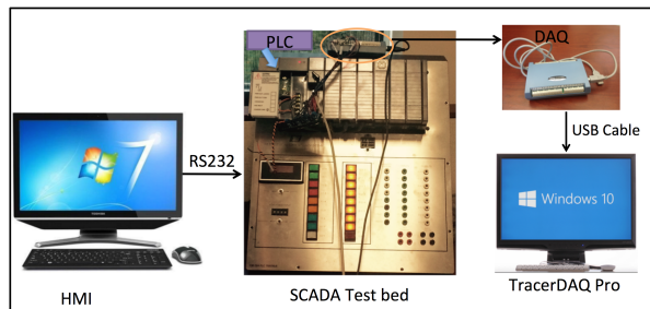
Figure 3: SCADA testbed
