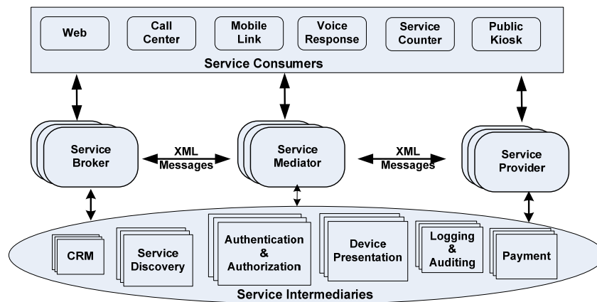
Figure 1. Top-level Architecture of a Service Ecosystem (Barros & Dumas 2006).
