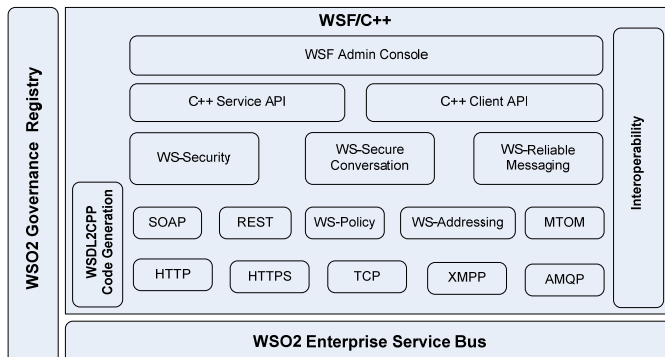
Figure 5. WSO2 WSF.
