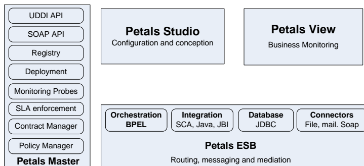
Figure 4. Petals WSF.
