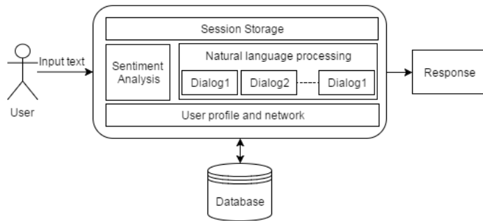
Figure 1. General architecture of intelligent virtual assistant
