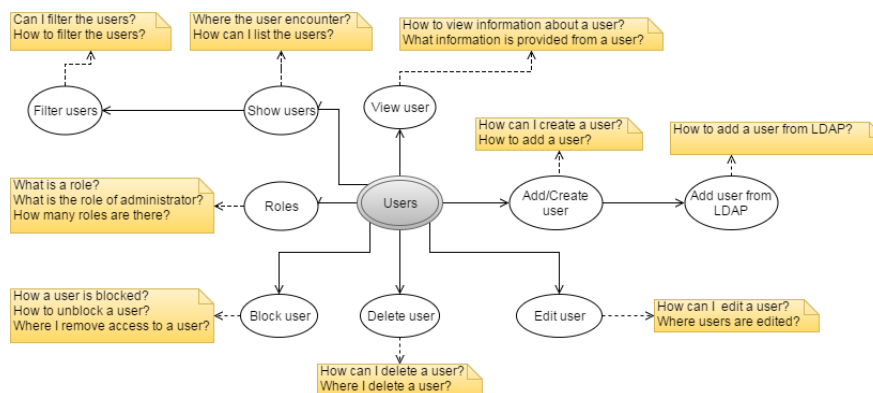
Figure 3. Diagram for the "Users" topic, and examples of questions to be answered.
