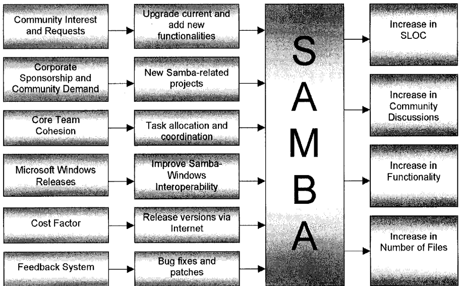
Figure 2: Samba's evolution.
