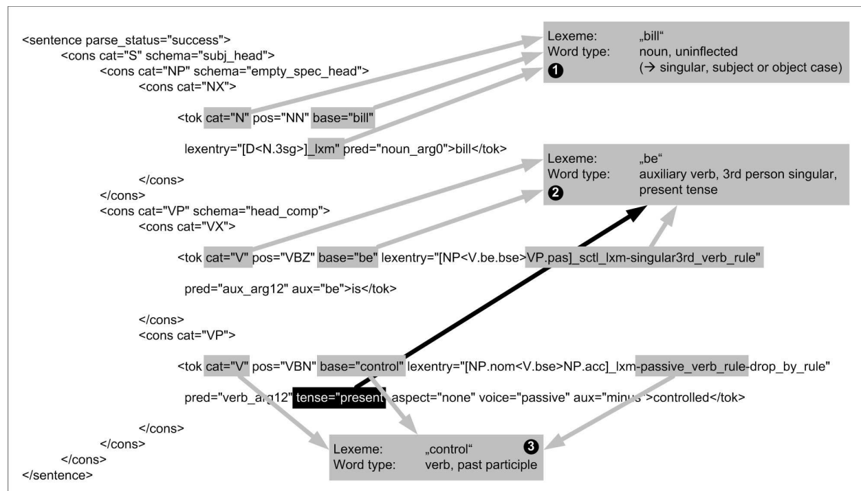
Figure 8: Exemplary Parsing Result
