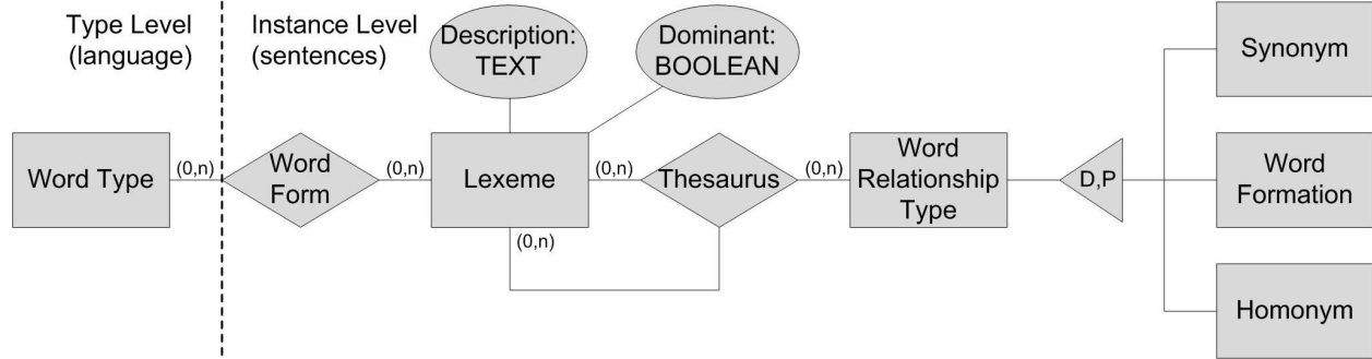
Figure 5: Specification of Term Conventions on Instance Level
