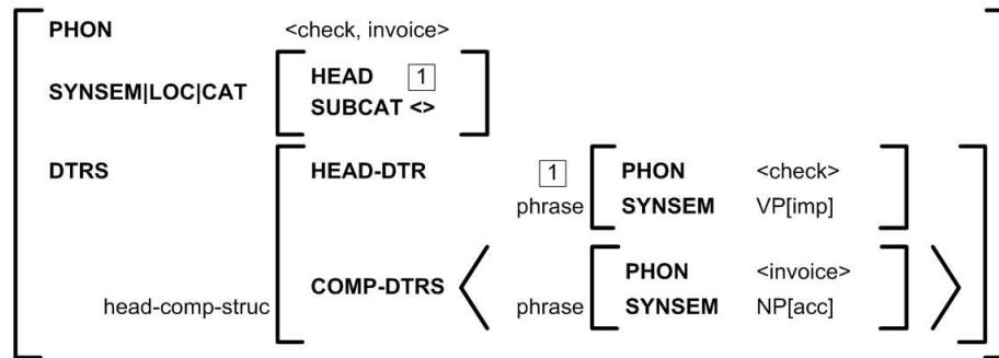
Figure 6: Exemplary HPSG Parsing Result
