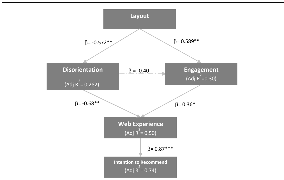
Figure 2: Regression Results, ** indicates p < 0.0001 , * indicates p < 0.001 , + indicates p < 0.05 , + indicates almost significant ( p = 0.058 )
