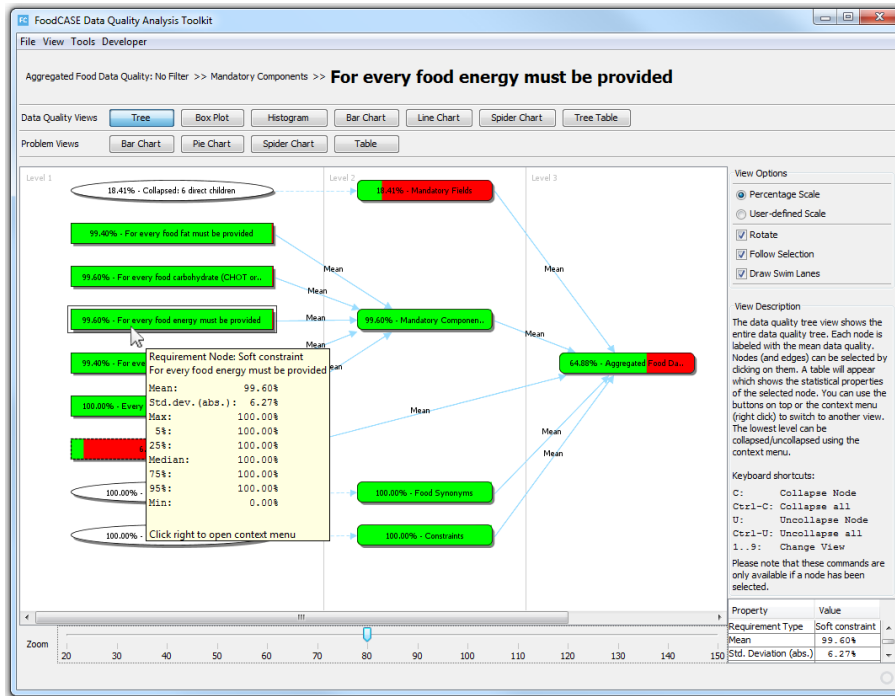
Figure 4: Tree visualisation of DQAF
