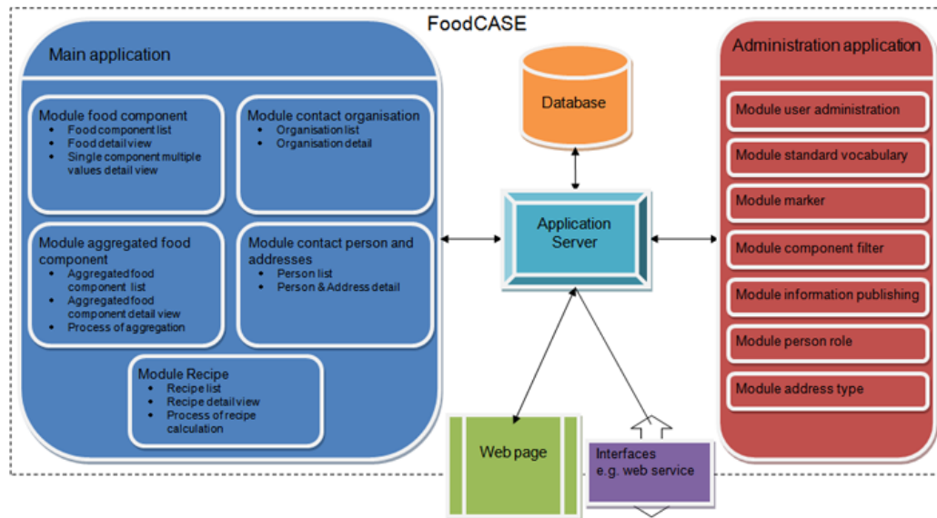
Figure 6: Architecture of the FoodCASE system. The six modules are highlighted in different colours.
