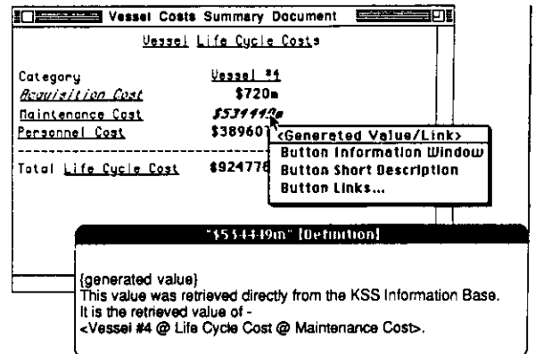
Figure 4. Selecting $534449 (the Maintenance Cost for Vessel #4) causes a "pop-up menu" to appear with valid operations for the selection. Note that key words are underlined in the document, generated values are boldface and links are italicized.
