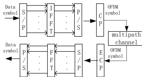
Figure 2. Baseband OFDM System
