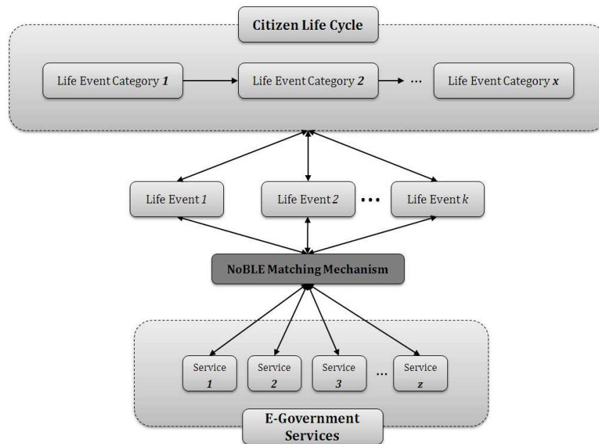
Figure 1: Hierarchical structure of NoBLE framework
