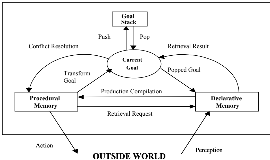
Figure 1. ACT-R
