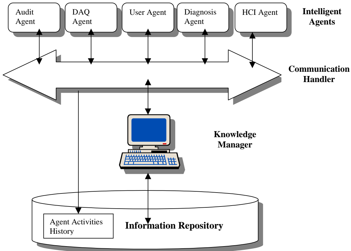
Figure 1 The generic multi-agent architecture for Internet security
