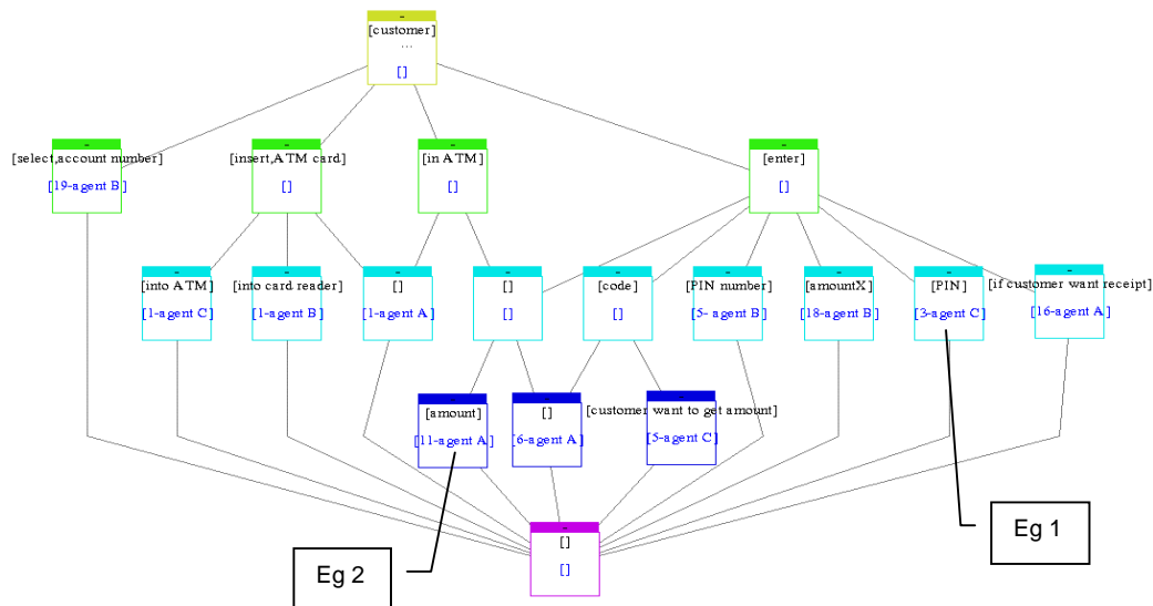
Figure 2: The concept lattice for the question “what is the customer involved in?” for the ATM example
