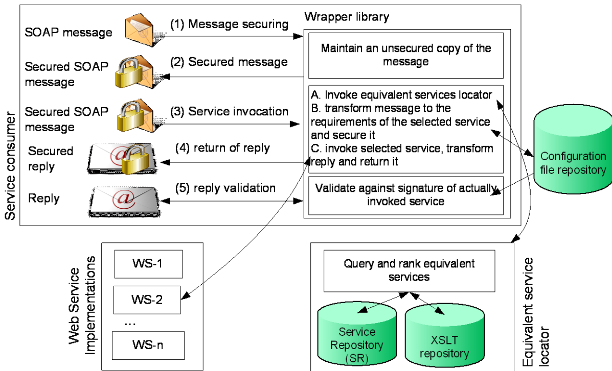
Figure 78. Overall architecture of the secure services adaptation framework
