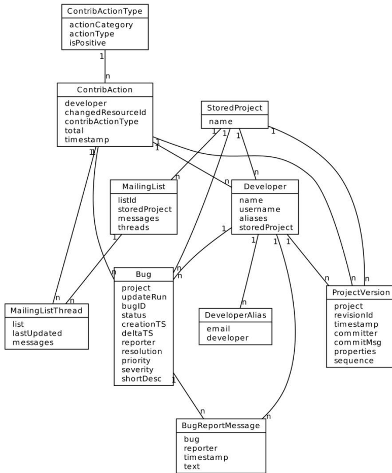
Figure 1. Relationships between entities defined by the Alitheia Core storage schema and those defined by the contribution plug-in
