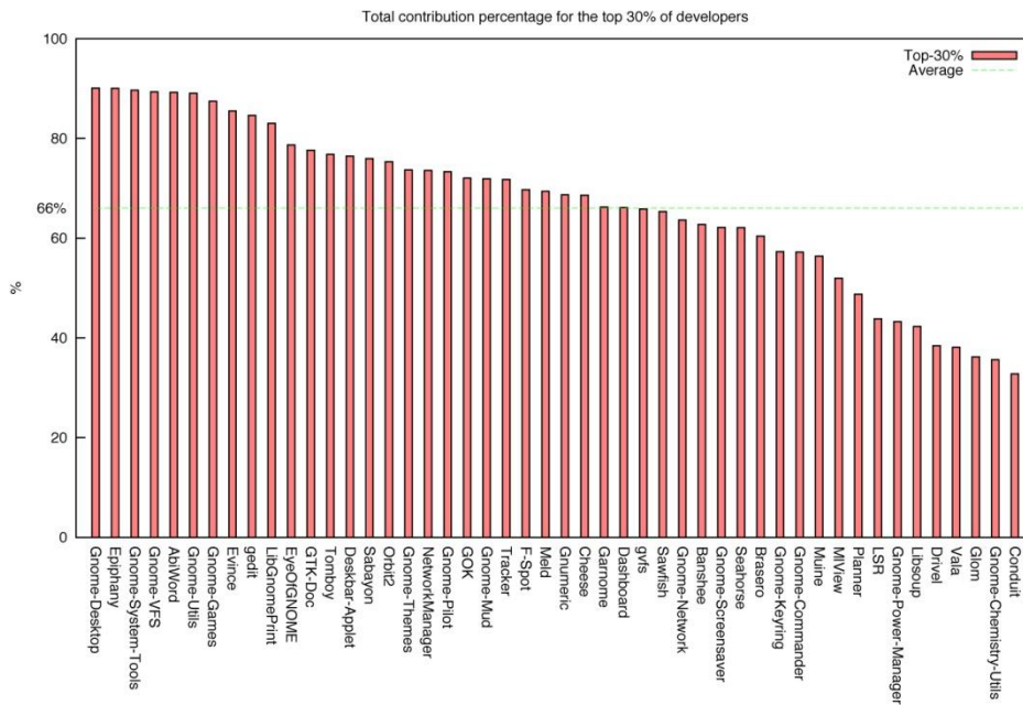
Figure 37. Total contribution from the top 30% of developers for various projects
