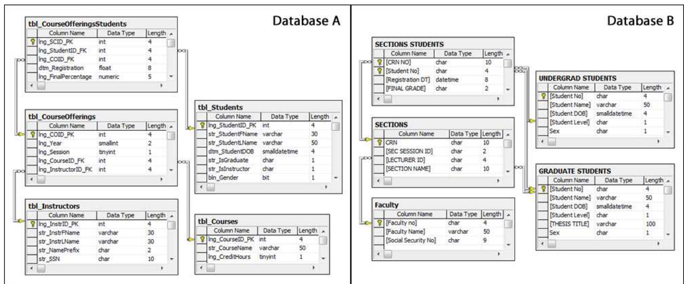
Figure 1. Two hypothetical databases belonging to the same domain that require integration
