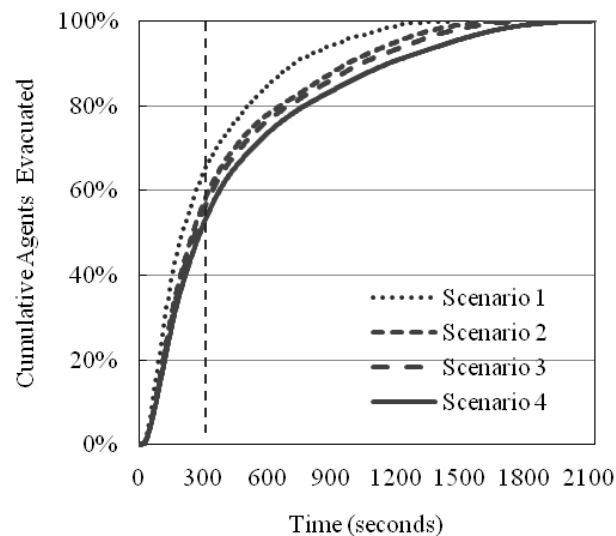
Figure 3. Mean Evacuation Curves for all Agents
