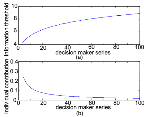
Figure 2. (a) Information threshold, (b) n^{\text{th}} decision-maker's contribution to information cascade.
