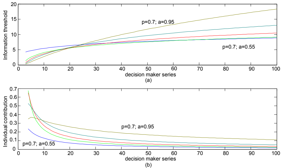
Figure 3. (a) Information threshold, (b) n^{\text{th}} decision-maker's contribution to information cascade while \alpha = 0.55 \sim 0.95 given p=0.7 .
