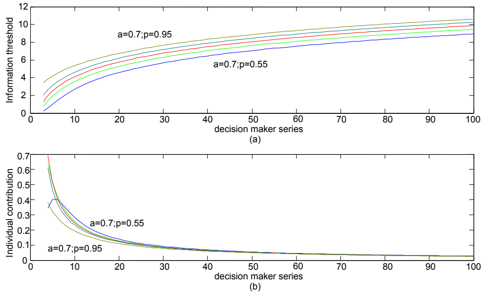
Figure 4. (a) Information threshold, (b) n^{\text{th}} decision-maker's contribution to information cascade while p=0.55\sim 0.95 given \alpha=0.7 .
