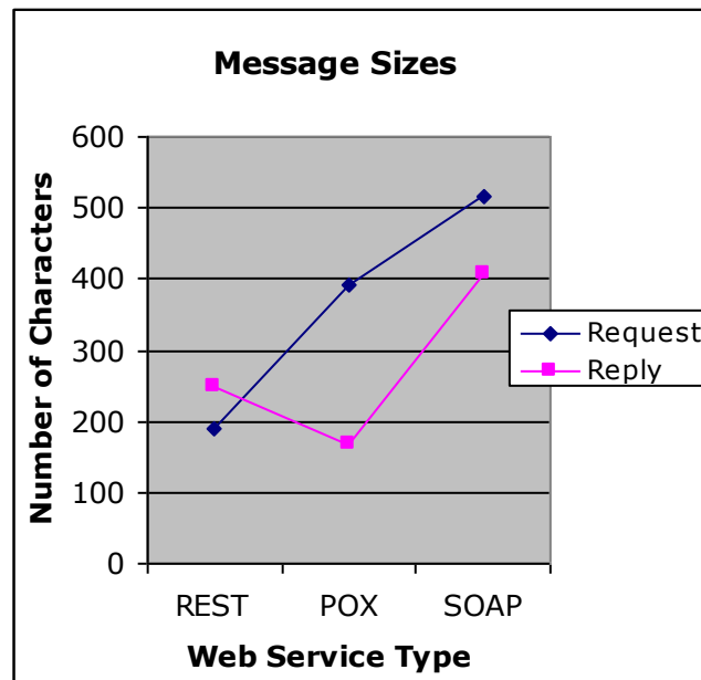
Figure 2 Message Sizes
