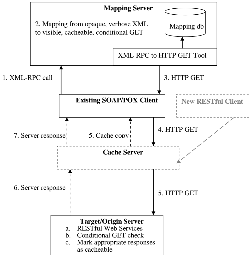
Figure 1 Framework Architecture
