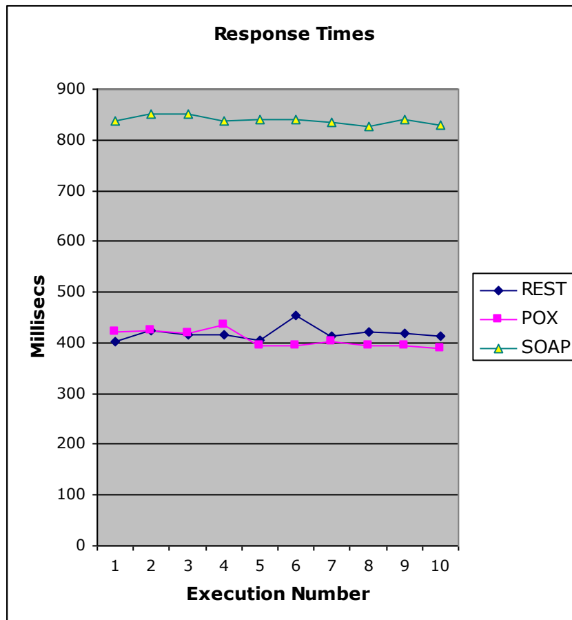
Figure 3 Response Times
