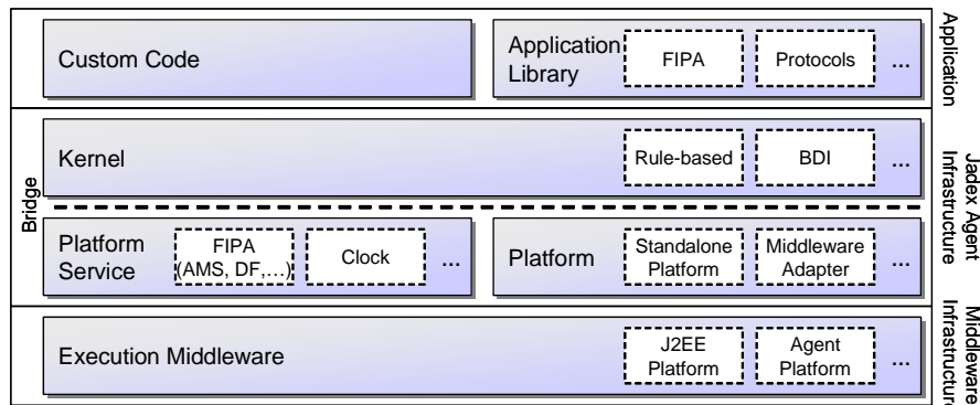
Figure 1: Jadex V2 architecture
