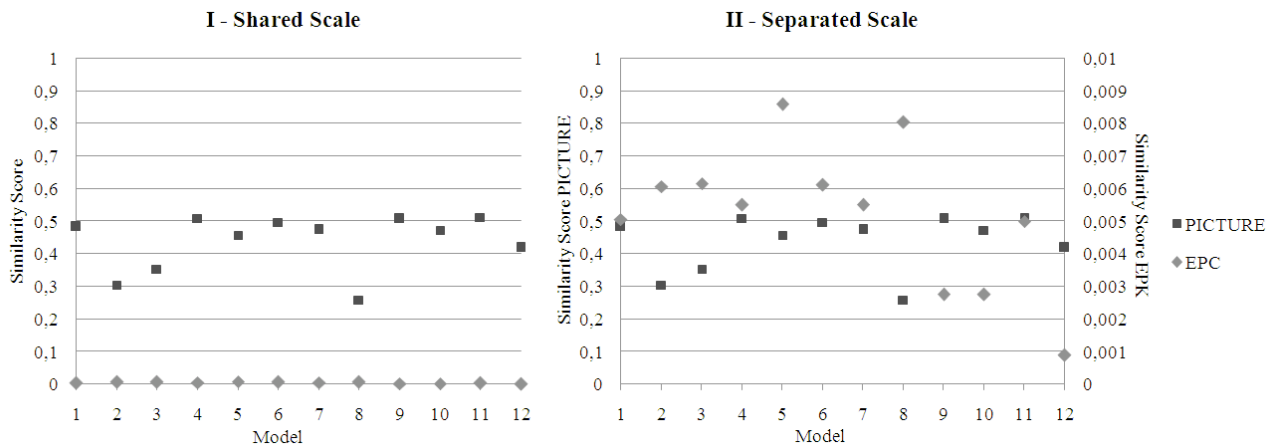
Figure 1: Average similarity degrees for PICTURE and EPC models
