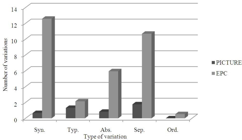
Figure 2: Numbers of variations for PICTURE and EPC according to the different variation types
