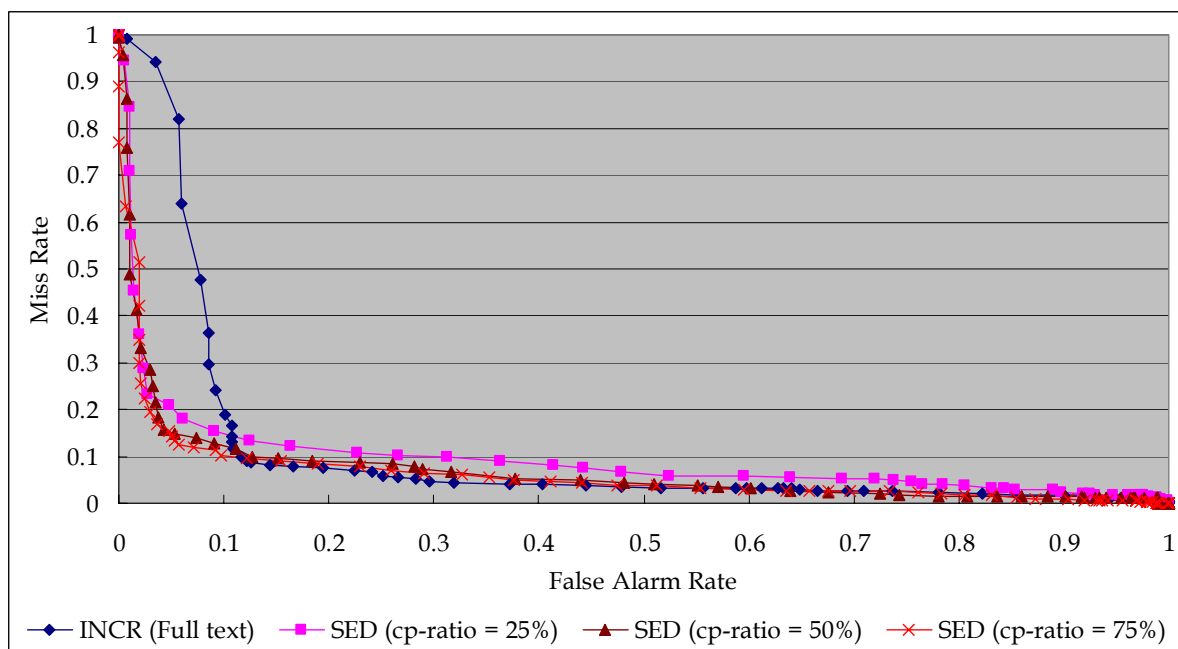
Figure 3: Detection Error Tradeoff Curves of Different Event Detection Techniques
