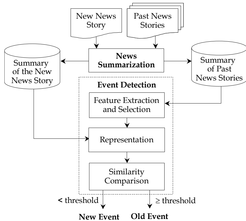
Figure 1: Overall Process of the SED Technique
