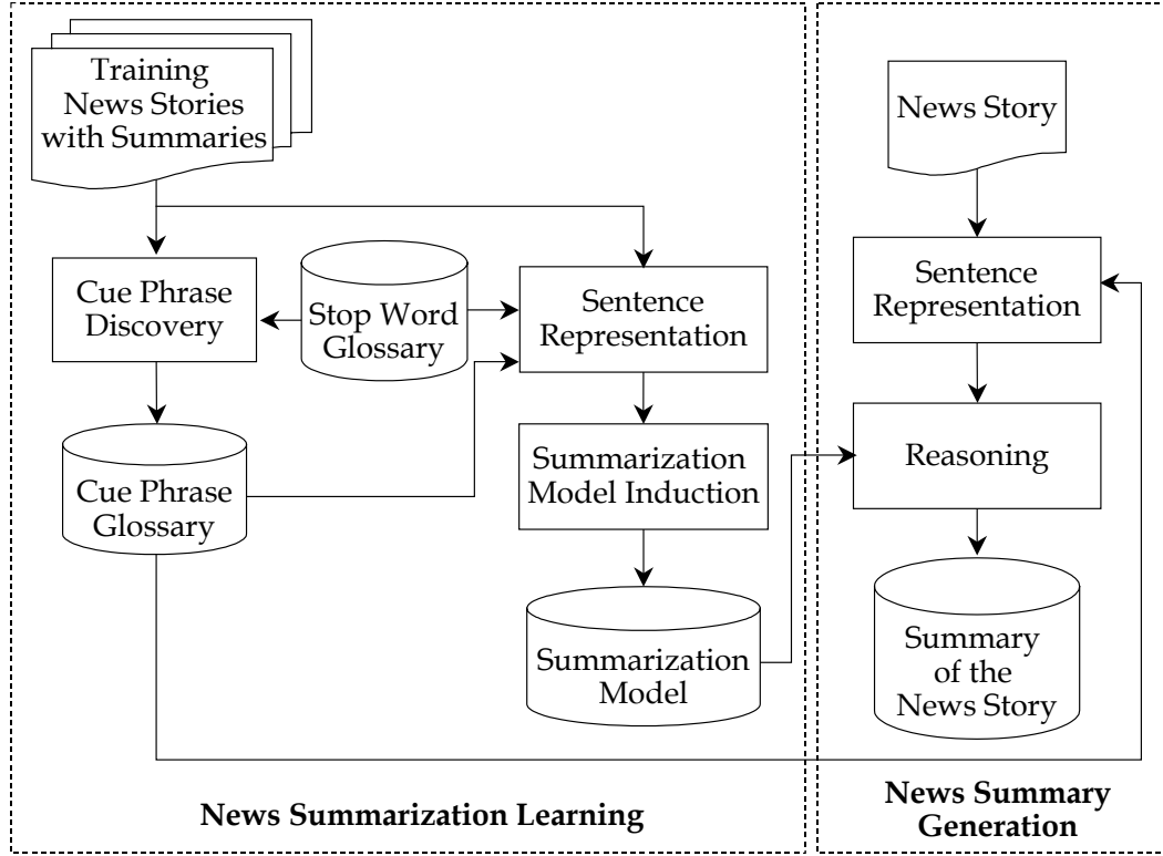
Figure 2: Process of News Summarization Phase
