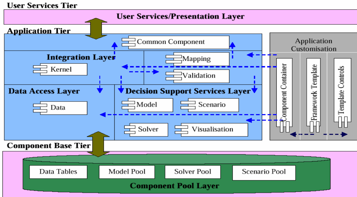
Figure 7: SDSSG Architecture
