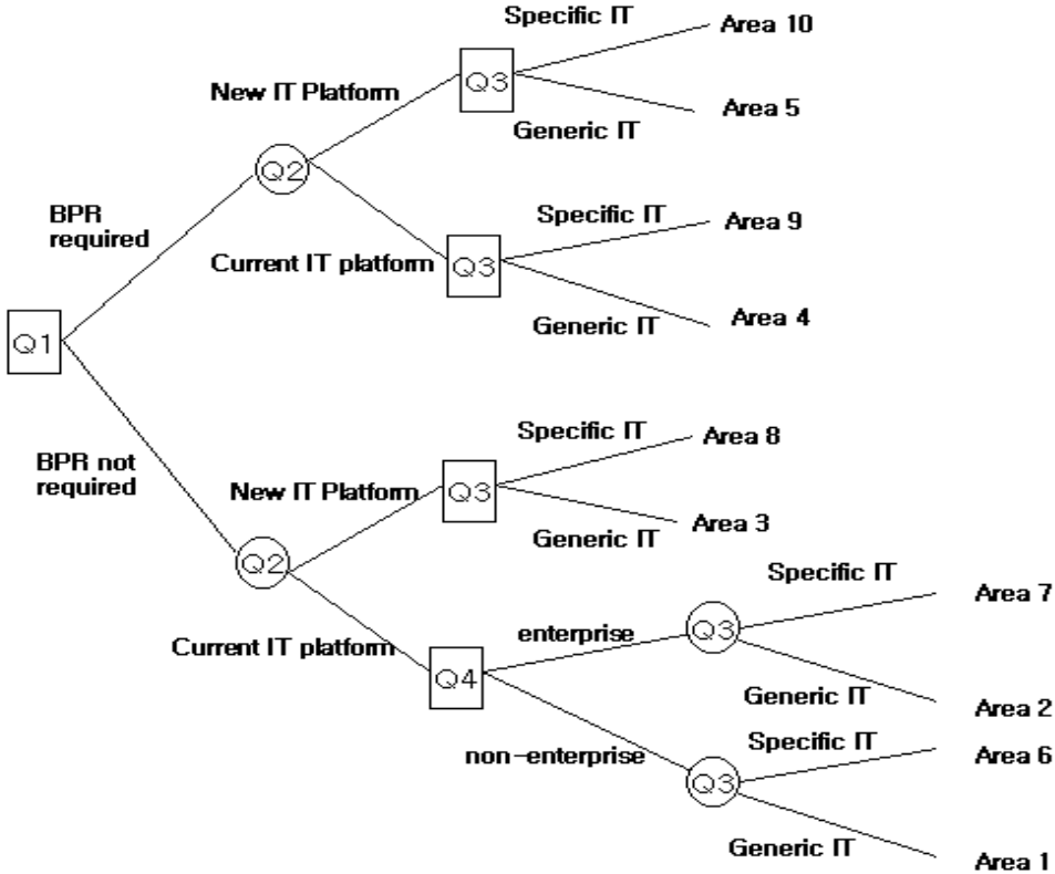
[Figure 2] Decision tree model for ISP methodology selection
