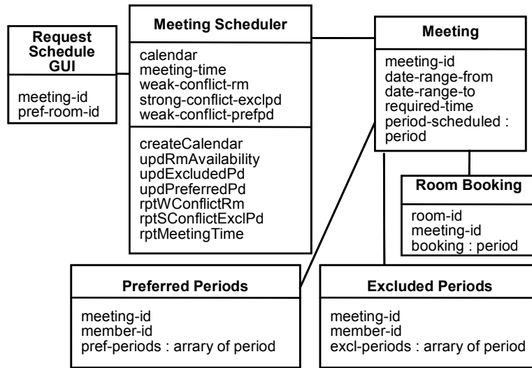
Figure 4. A Class Diagram for Automated Meeting Scheduler
