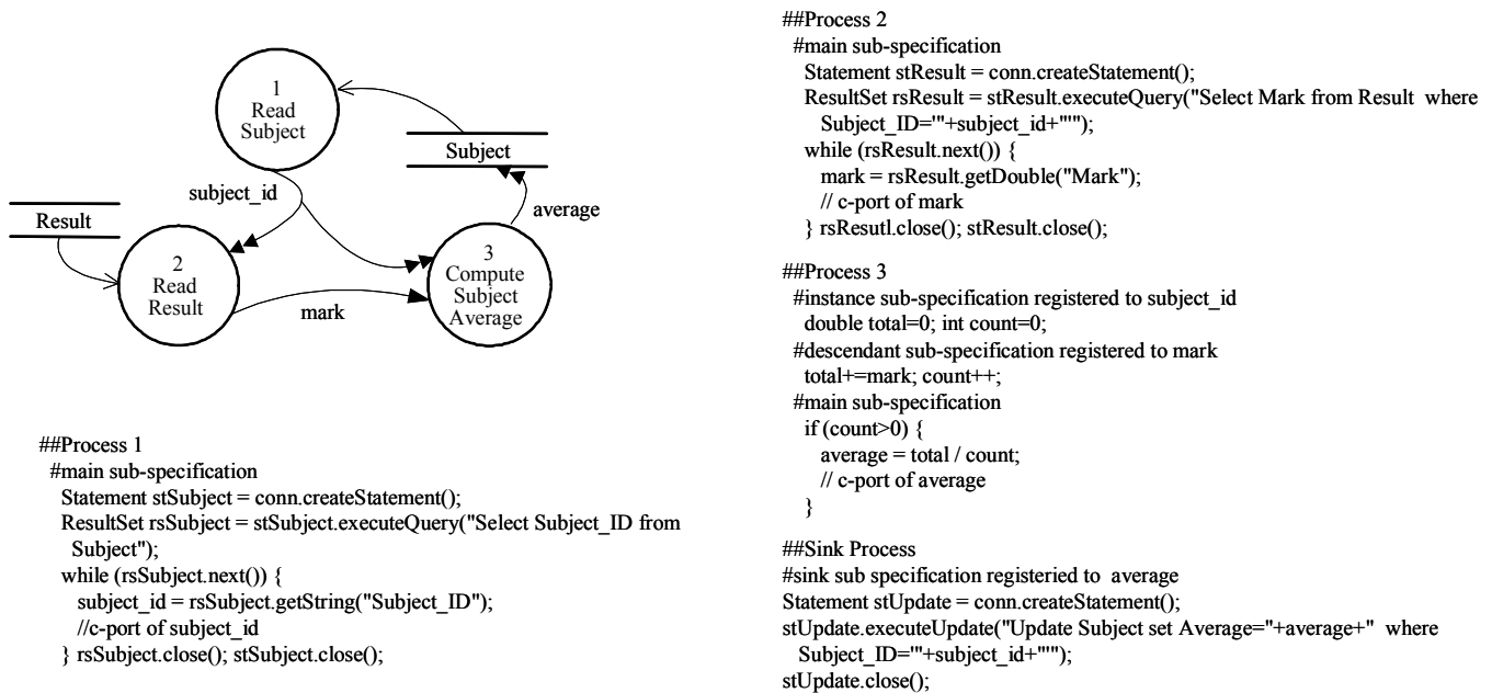
Figure 1. Update Subject Average DF Net
