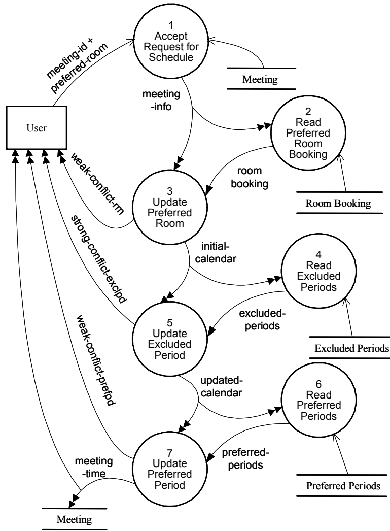
Figure 3. Schedule Meeting DF Net
