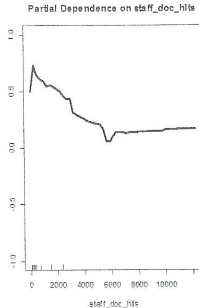
Figure 4: Partial dependence plot showing the effect of total staff hits to documents across all the students learning contexts on student progression
