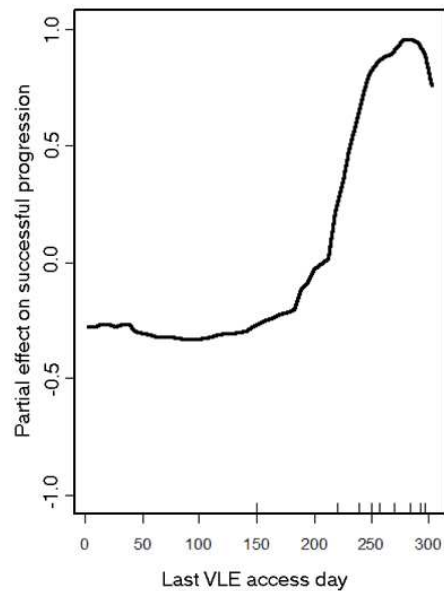
Figure 3: Partial dependence plot showing the effect of last access of VLE on student progression
