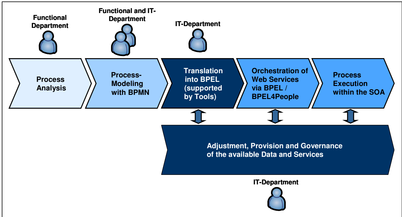
Figure 2. Integration of the functional department into the process design within an SOA
