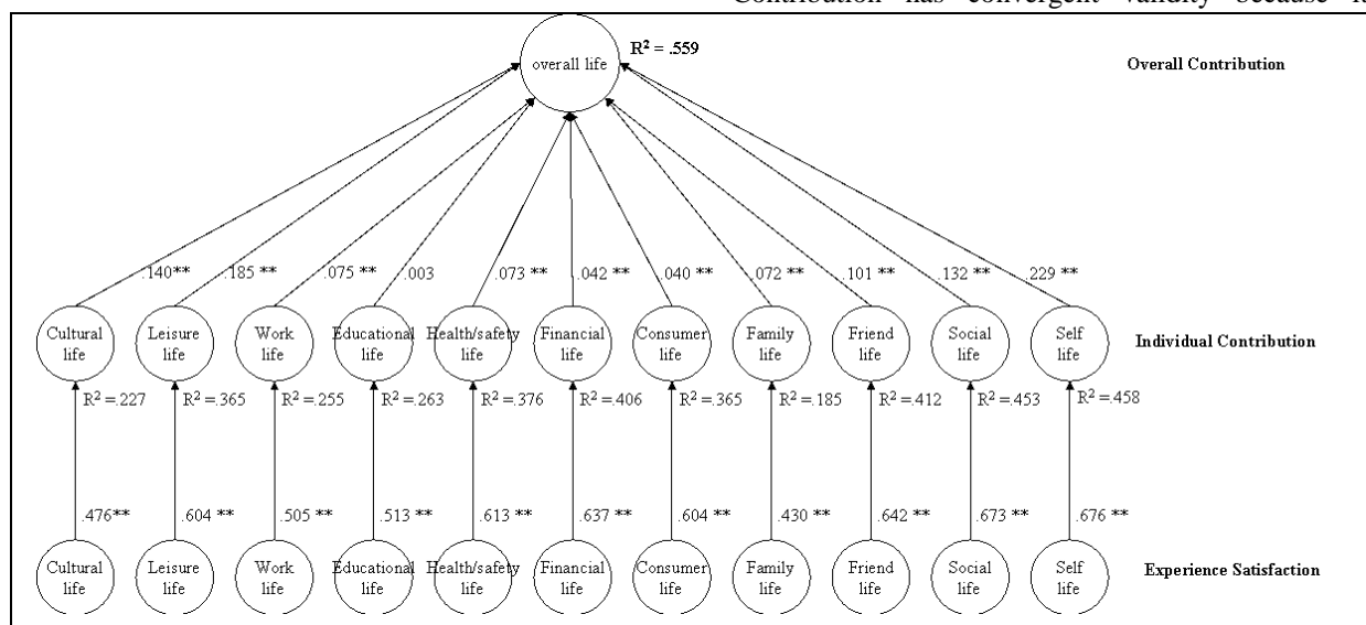
Figure 2. PLS results for research model verification
