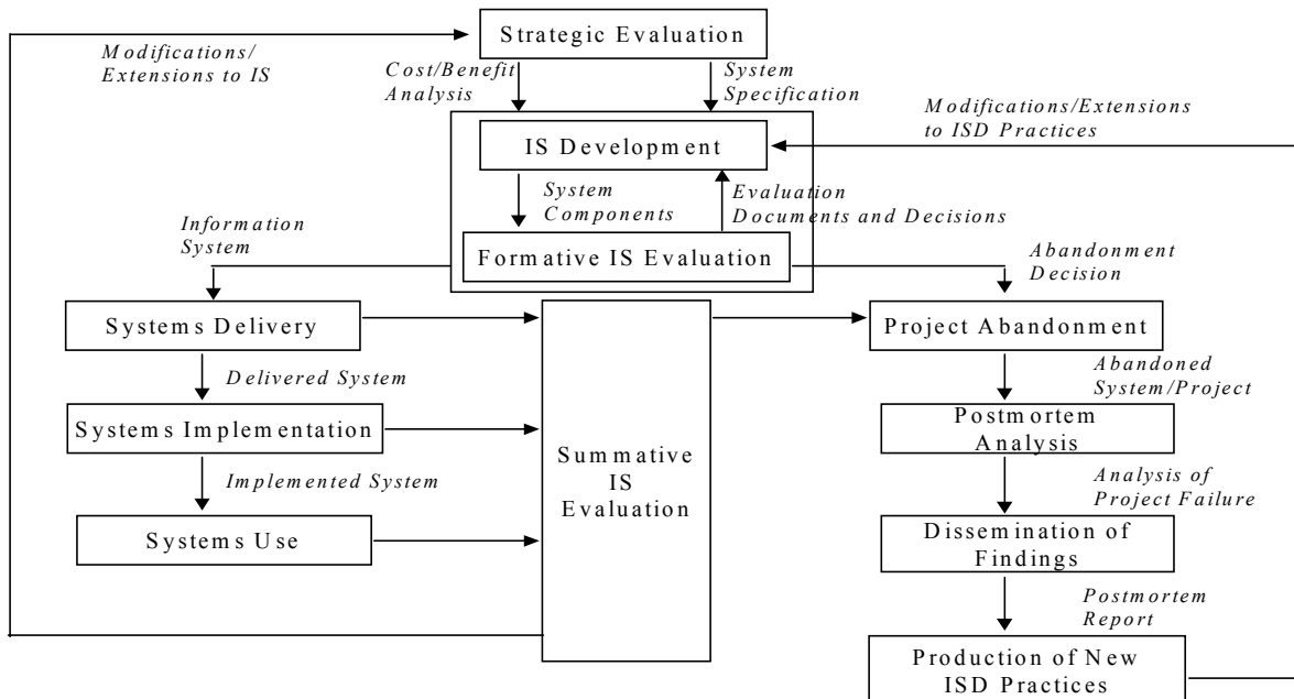
Fig. 1 IS Evaluation and Organisational Learning
