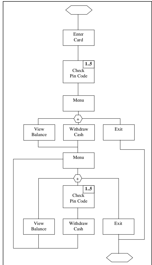
Fig. 5. Episode structure of cash withdrawal with an ATM
