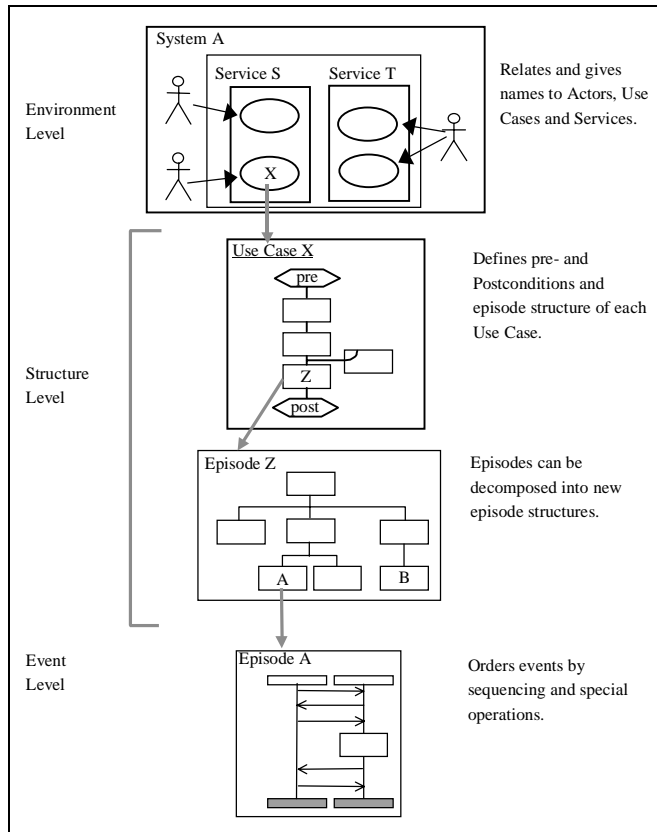
Fig. 1. Overview of the hierarchical use case model
