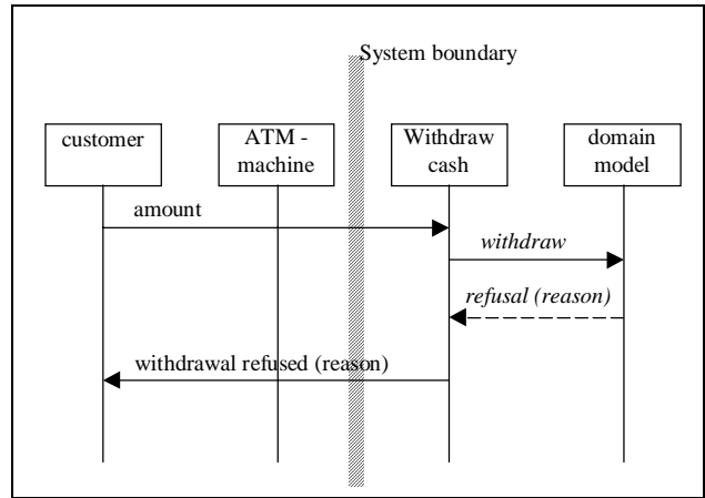
Fig. 9. Exception scenario for Withdraw_Cash
