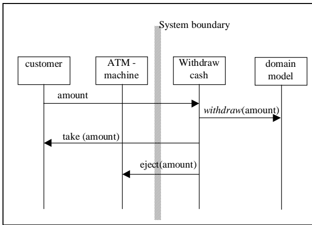
Fig. 8. Sequence chart for Withdraw_Cash
