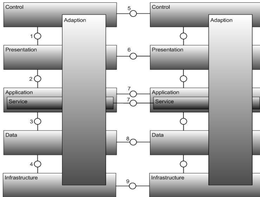
Figure 1: Adaptability Reference Model for ERP Systems
