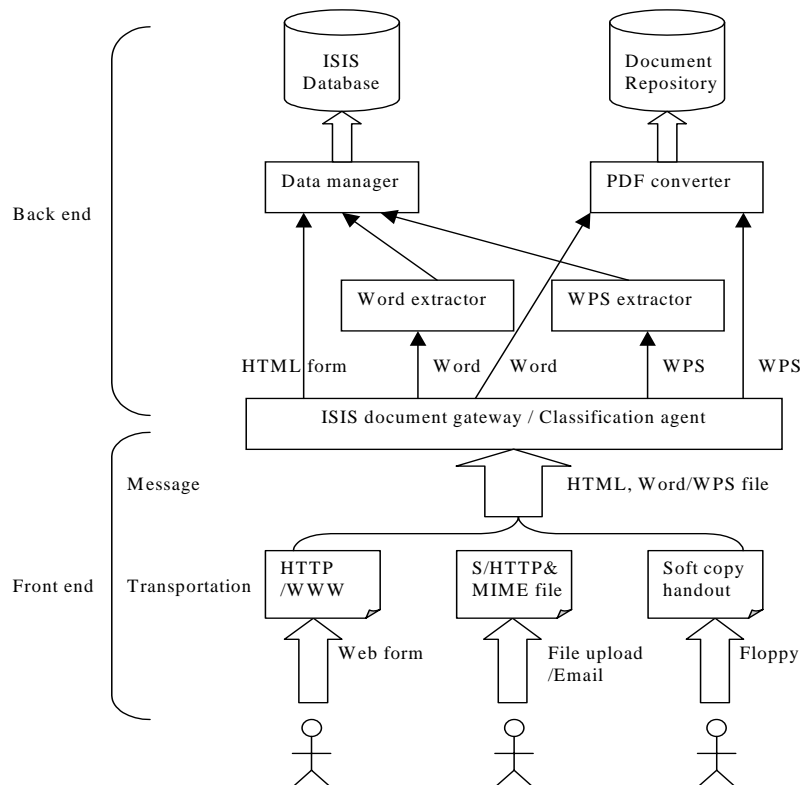
Figure 4. e-Document extraction and management architecture
