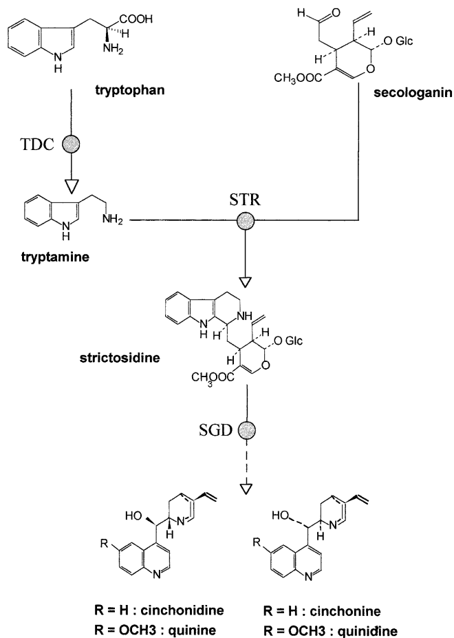
Fig. 1 Biosynthesis of quinoline alkaloids in Cinchona species. Dashed arrow indicates that the biosynthetic route(s) involved are not exactly known (TDC tryptophan decarboxylase, STR strictosidine synthase, SGD strictosidine \beta -D-glucosidase)
