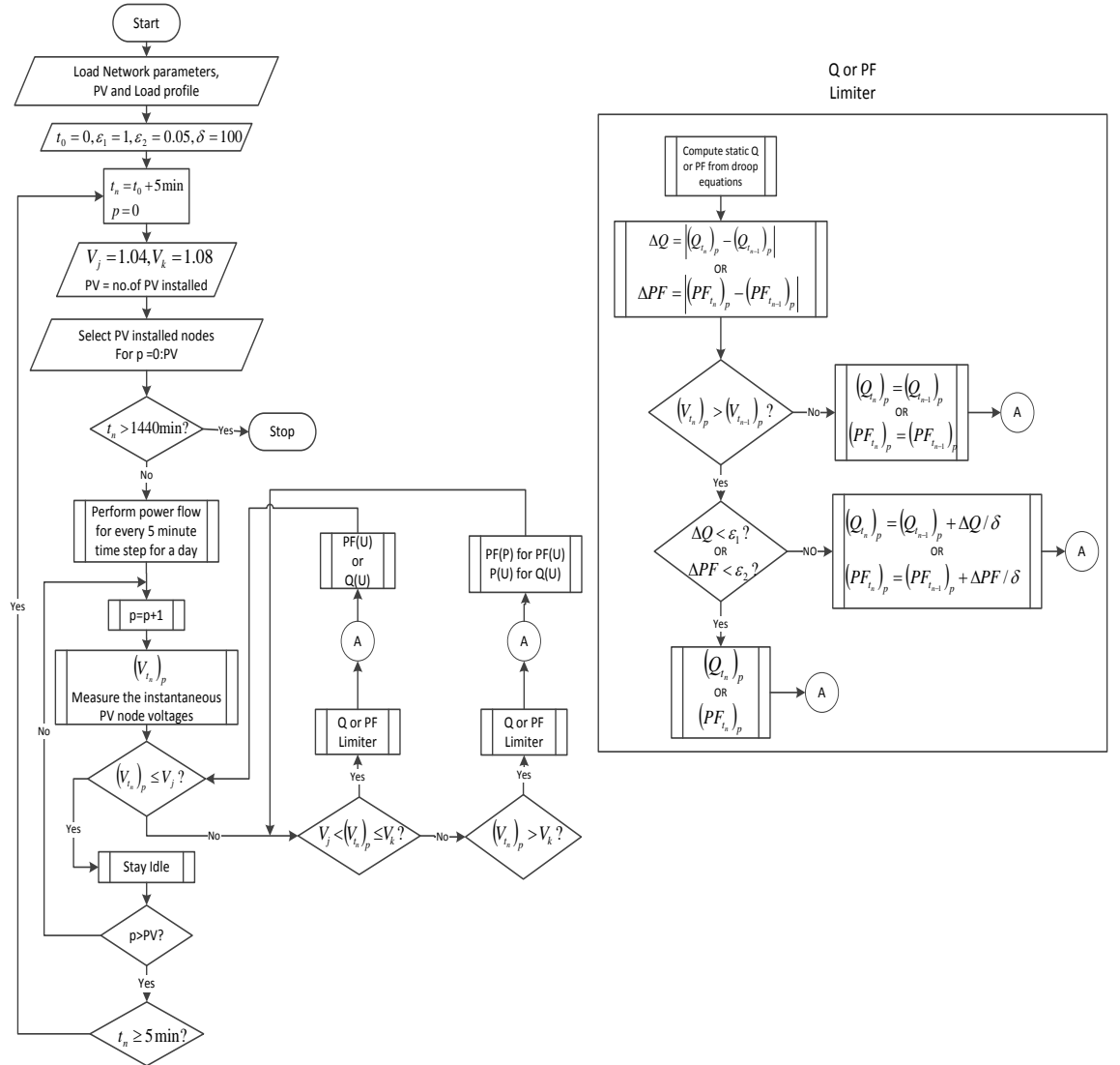
Figure 5.4 : Coordination algorithm
