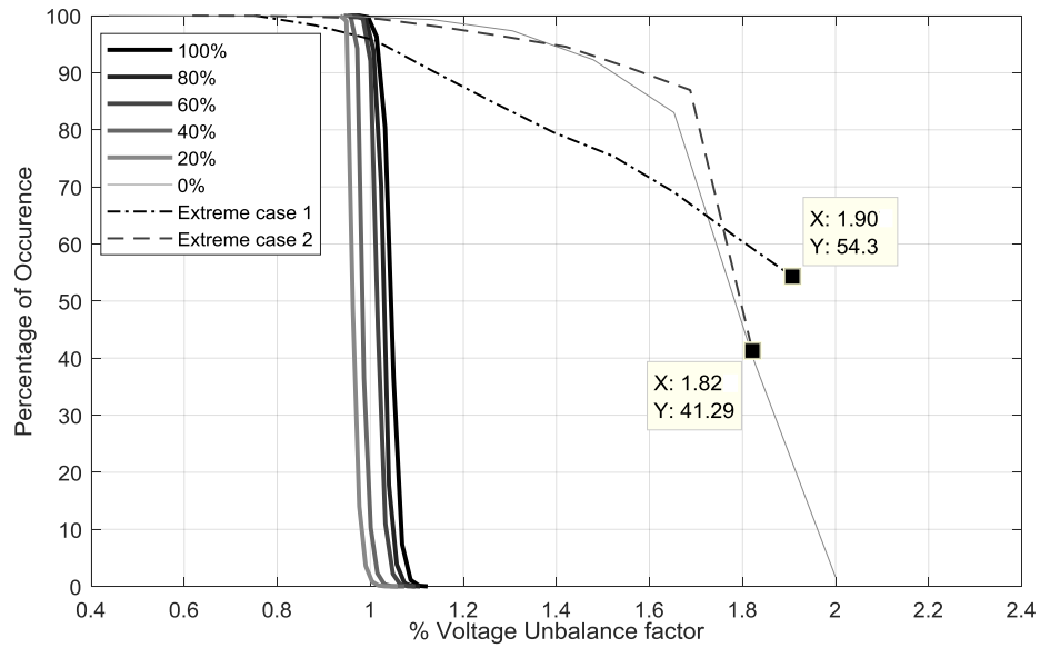
Figure 3.12 : Percentage of site voltage unbalance factor
