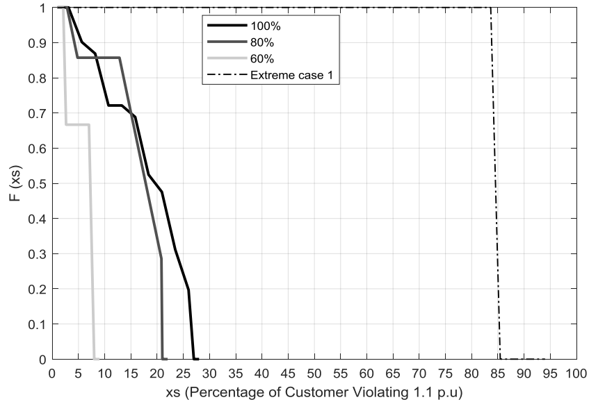
Figure 3.8 :CCDF of % of customer violating overvoltage
