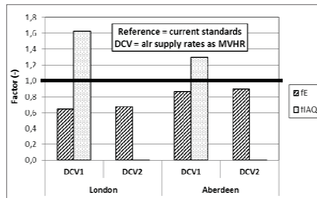
Figure 7: Heating energy ( f_E ) and IAQ ( f_{IAQ} ) factor for DCV1 and DCV2 for London and Aberdeen with adapted DCV air supply rates
