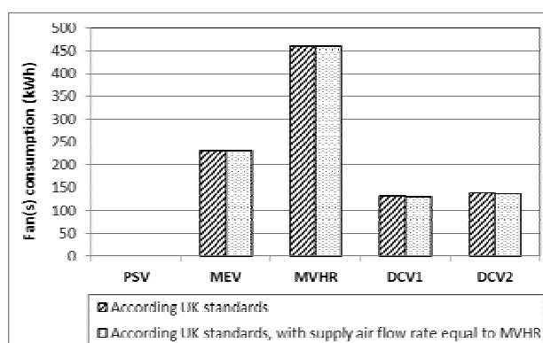
Figure 8: Annual fan(s) electricity consumption for the several mechanical ventilation systems for the location of London at a building air tightness of 3 \text{ m}^3/\text{h} \cdot \text{m}^2 , according to UK standards (left) and with adapted air supply rates (right)
