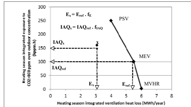
Figure 3: Heating energy and IAQ factor calculation for a ventilation system 'x' with respect to reference systems
