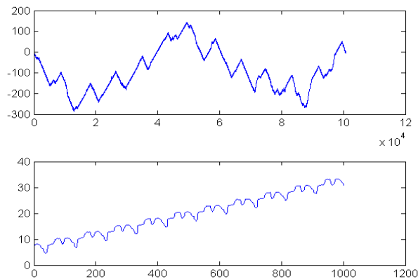
Figure 1: Unwrapped and de-trended phase for a concert A recorded from a violin (above) and a windowed sample of the signal (below) showing a series of replica phaselets associated with the primary resonance characteristics of the instrument.
