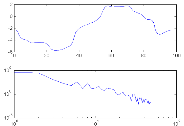
Figure 2: Isolated phaselet (above) and the associated log-log power spectrum (below).
