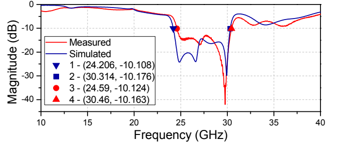
Fig. 3. Measured and simulated S11 (matching) for the Vivaldi antenna showing good matching from 24 GHz to 30 GHz.
