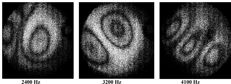
Fig. 3. ESPI vibration modes of an aluminium diaphragm. The amplitude of the sinusoidal signal driving the loudspeaker is 1 V. The field of view is 40 mm x 40 mm.
