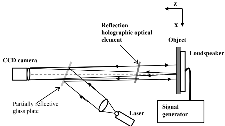
Fig. 2. ESPI system with a holographic optical element and a partially reflective glass plate
