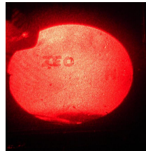
Fig. 1. A typical reconstructed image from a reflection hologram. The diffraction efficiency (defined as the ratio of diffracted light intensity to incident) is above 50%.
